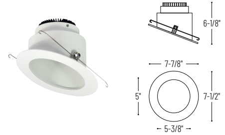
NRM2-6S11 Slope Open Reflector
