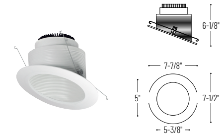
NRM2-6S12 Slope Baffle
